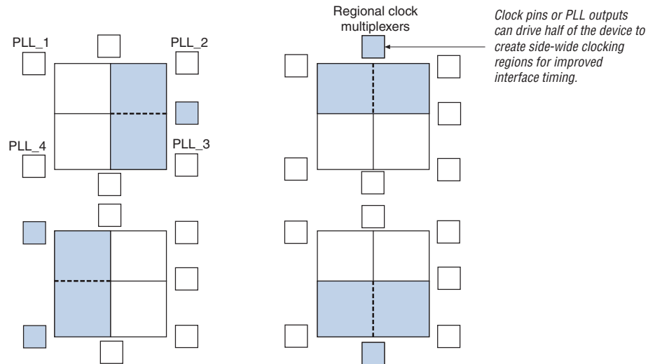
Figure 5-10. Device Dual-Regional Clock Region for Arria II GX Devices
