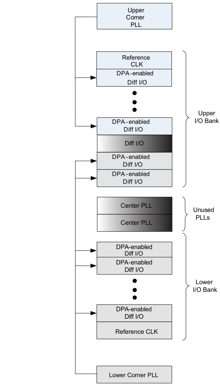
Figure 8-26. Corner PLLs Driving DPA-Enabled Differential I/Os
