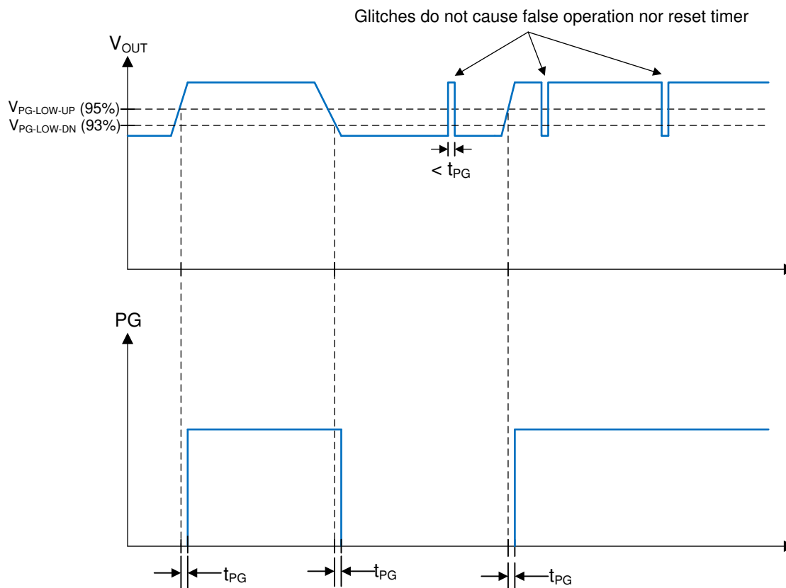
Figure 7-2. Power-Good-Timing Behavior
