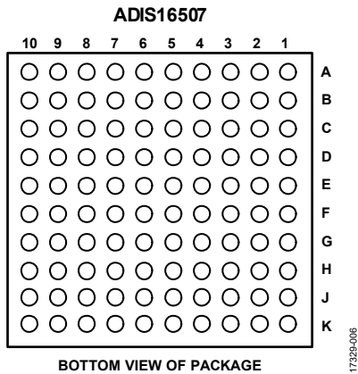
ADIS16507 BOTTOM VIEW OF PACKAGE Figure 5. Pin Assignments, Bottom View
