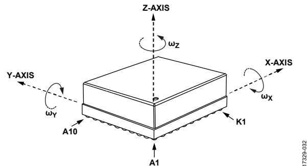
Figure 49. Gyroscope Axis and Polarity Assignments
